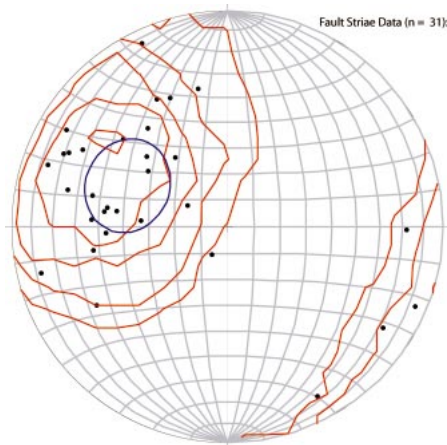
Figure 2. Scatter plot of fault striae for the Manly Pass fault zone in the northern part of the Slate Range. Mean vector plunges 48° toward 292°. Red lines are Kamb 2% contours (maximum = 10%). Blue oval is 95% confidence area for mean vector (radius is 17°).
